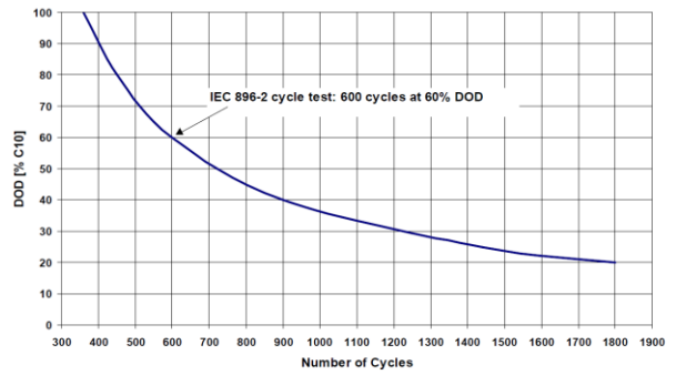
Cycle Life
