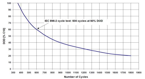
Cycle Life
