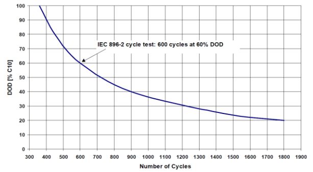
Cycle Life
